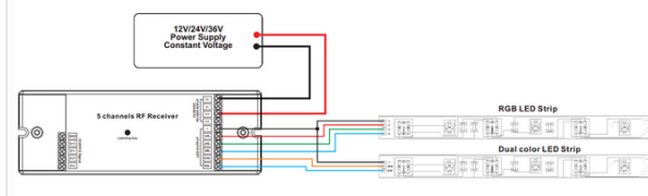
Wiring Diagram
