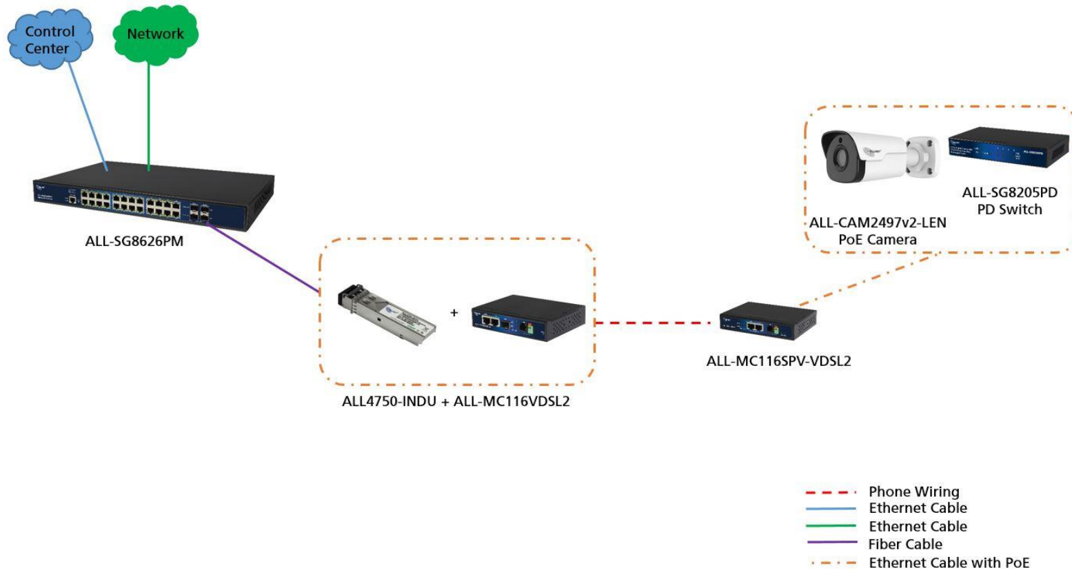
Figure 2.2 Application Diagram
