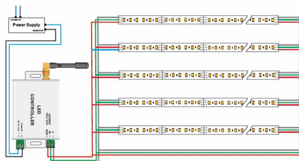
How to connect Flexible strip
