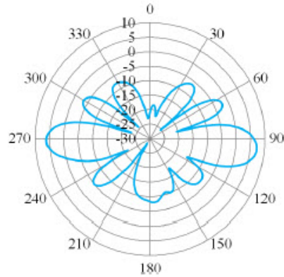
— 868MHz Vertical
