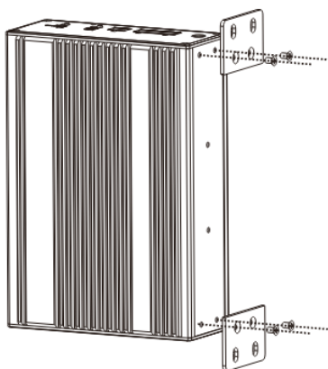
Wall installation
