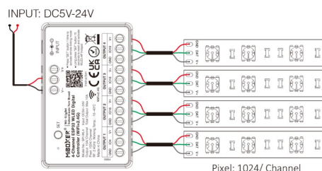
Connection Diagram
