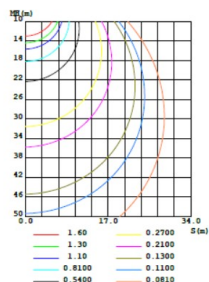
C0 PLANE ISOLUX DIAGRAM (UNIT:lx)
