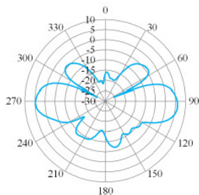
— 868MHz Vertical
