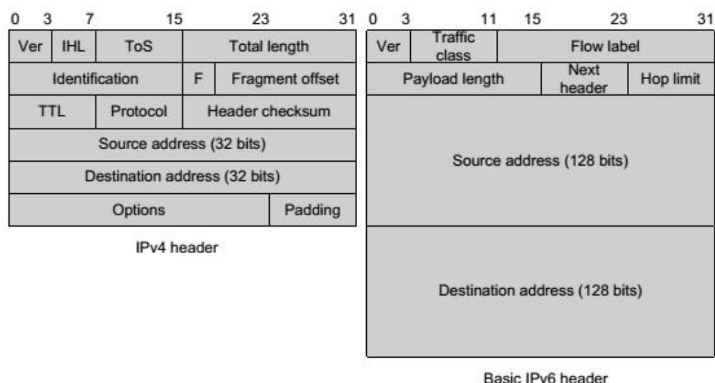
Figure 1 comparison of IPv4 header and IPv6 basic header format
