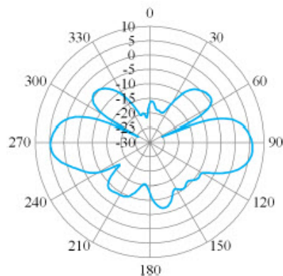
— 868MHz Vertical
