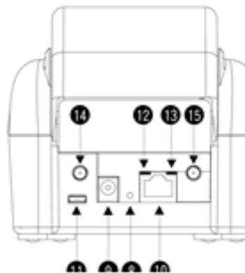
Rear Panel
