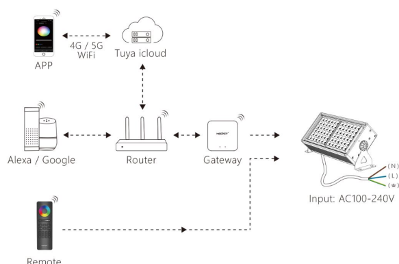
Application Diagram
