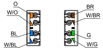
Double gang module carrier UP/0 flex
