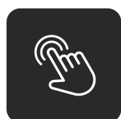
One-button Deployment
