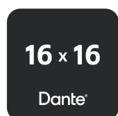
16*16 Dante Channel
