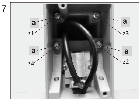
Lamp holder fixed ready by step
